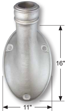
EDO 3" Diameter Poles Only* 30° Angle Only
