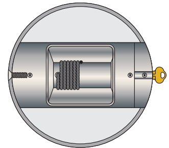
M-WINCH DETAIL
