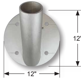
ECOST & ECOS 3" Diameter Poles Only 45° Angle Only
